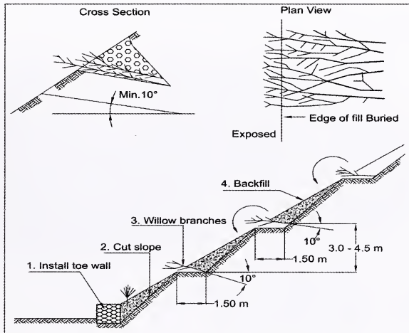
Fig. 17 (a) Brush Layering Process
