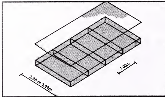
Fig. B - Gabion Mattress Unit
