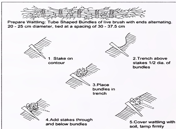
Fig. 16 (a) Contour Wattling Process
